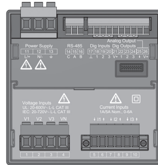
Fig. Rear of UMG 96-PQ-L
