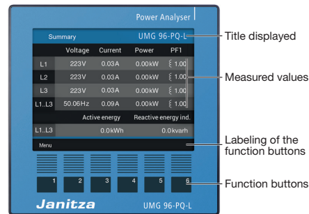
Fig. Standard display of UMG 96-PQ-L "Overview" measuring display
